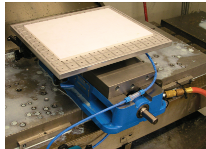
*真空吸盤VM100 (45375)與治具VM300 (45150)
