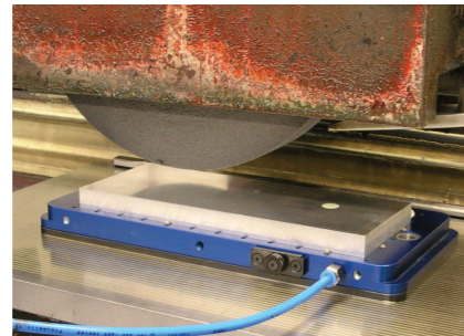
*真空吸盤VM100 (45375)在磁盤上
